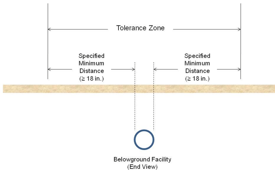
Figure 5 Tolerance Zone
