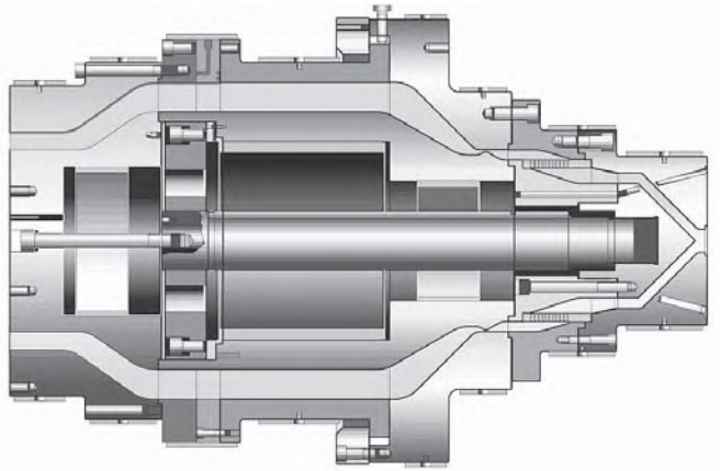
Figure 5.2 Pipe Die with Basket Design
