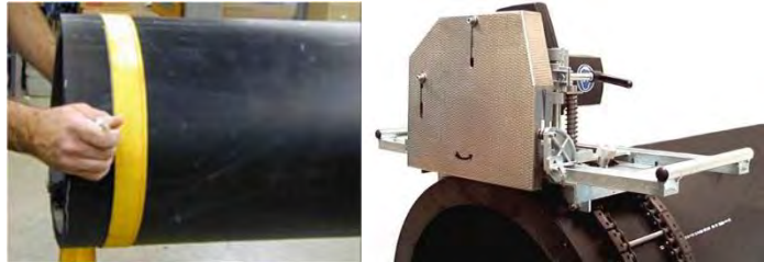
Figure III-c – Marking and cutting larger diameter pipes
