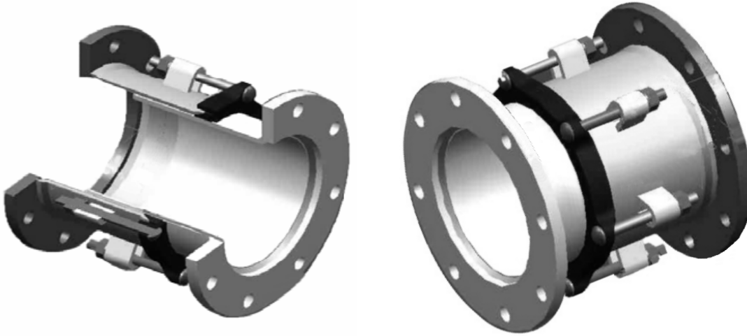
Figure 15 Dismantling Joint
