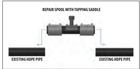
Fig. 5 Pipe Section Replacement with Tapping Tee
