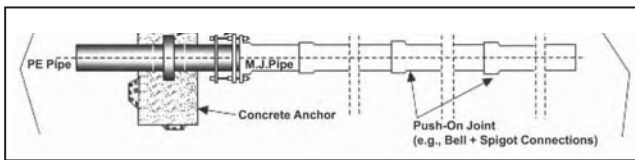
Figure A1 Pullout Prevention Technique
